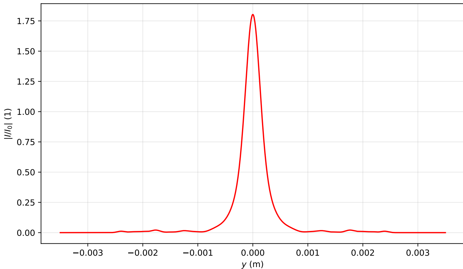
Intensity profile I(x=0, y, z=3.105)/I_0 , P_{in}=2.5P_{cr} , artificial time
